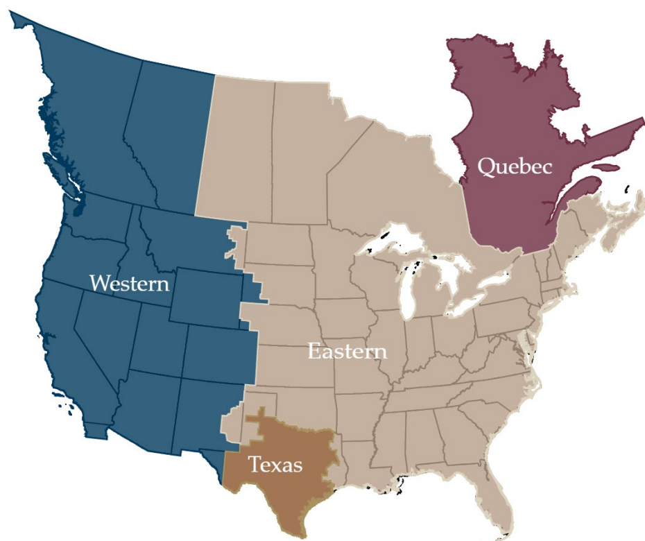
Figure 5: Four North American Electricity Interconnections Map. Source: WECC.org
