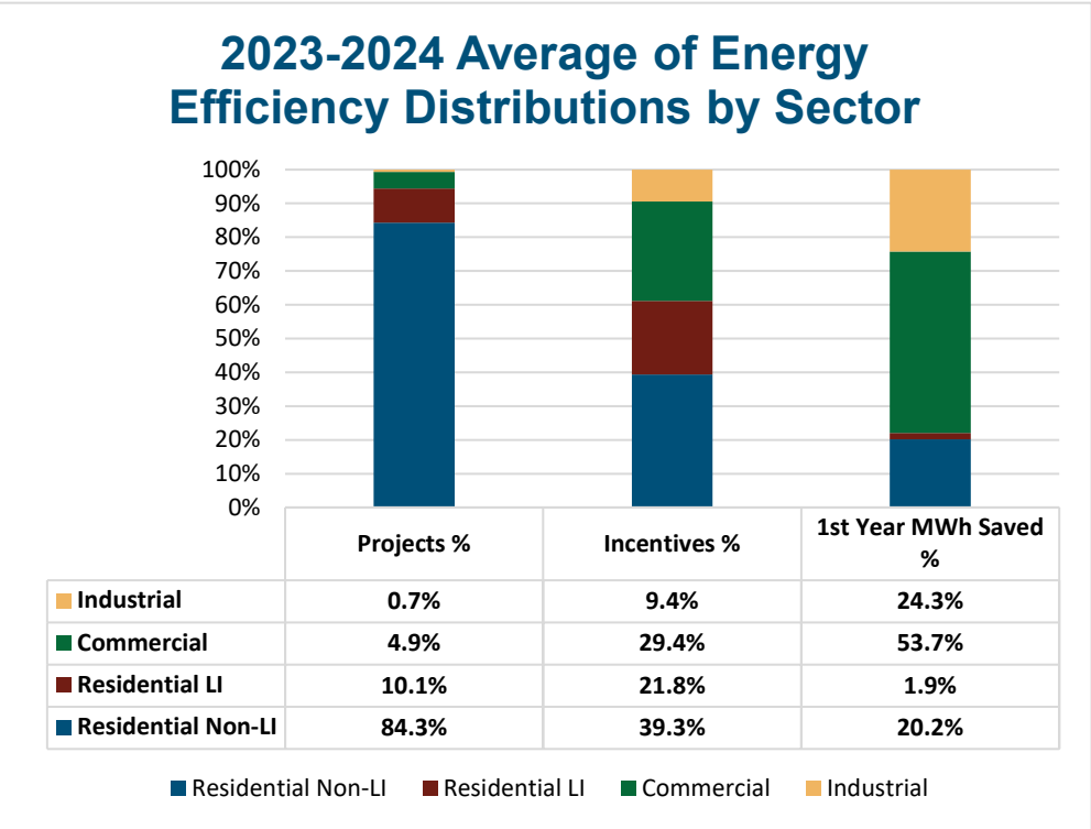
Figure 14: 2023-2024 Average Energy Efficiency Distributions by Customer Sector including Industrial, Commercial, Residential Limited Income, and Residential Non-Limited Income
