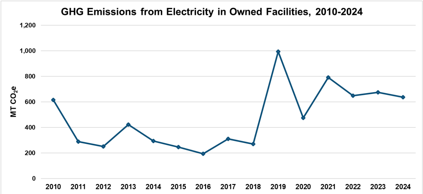
Figure 32: EWEB Emissions from Electricity Consumption (MT CO 2 e), 2010-2024
