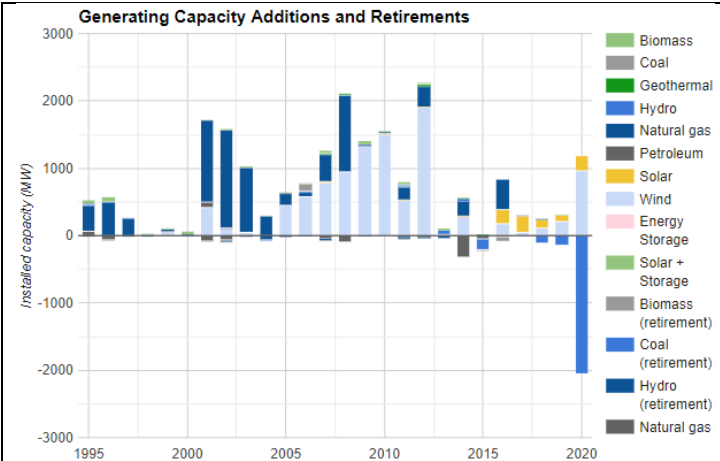
Figure H - Generation capacity additions and retirements
