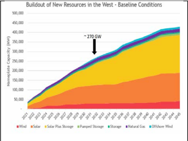
Figure I - Buildout of new resources in the west
