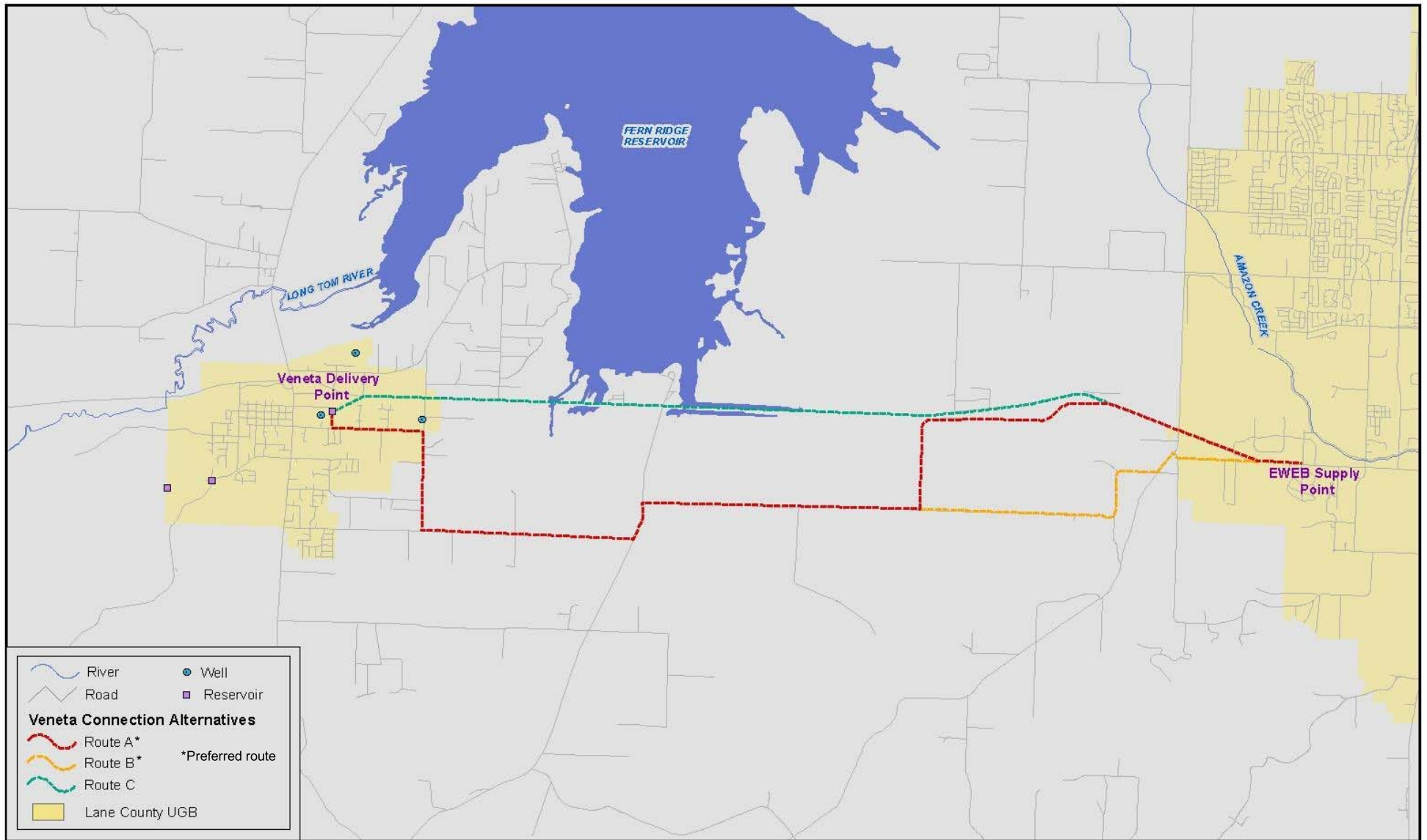
Figure 3 Veneta-EWEB Connection Alternatives for Water Supply
